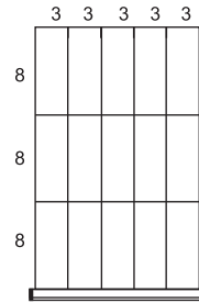
15 COMPARTMENTS L__BG-A0410__
