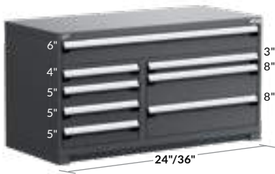
8 DRAWERS R5KKE-3007 60" x 24" x 32" R5KKG-3007 60" x 27" x 32"
