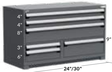
6 DRAWERS R5KJE-3003 54" x 24" x 32" R5KJG-3003 54" x 27" x 32"
