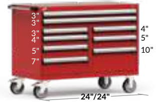
9 DRAWERS R5GHE-3009 48" x 24" x 37 1/2" R5GHG-3009 48" x 27" x 37 1/2"
